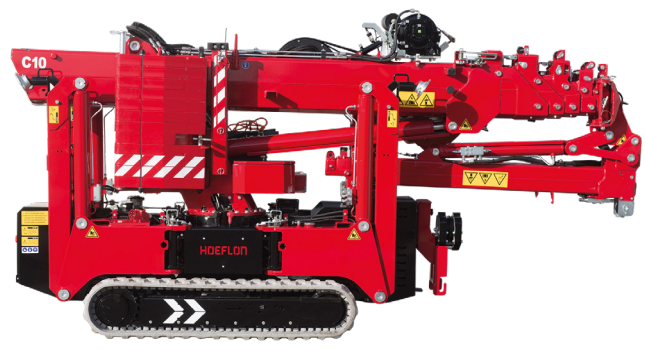
Available as both a hybrid (diesel + electric) and as a pure Power battery crane.
